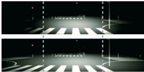
"Super Wide Range HID"-Scheinwerfer
